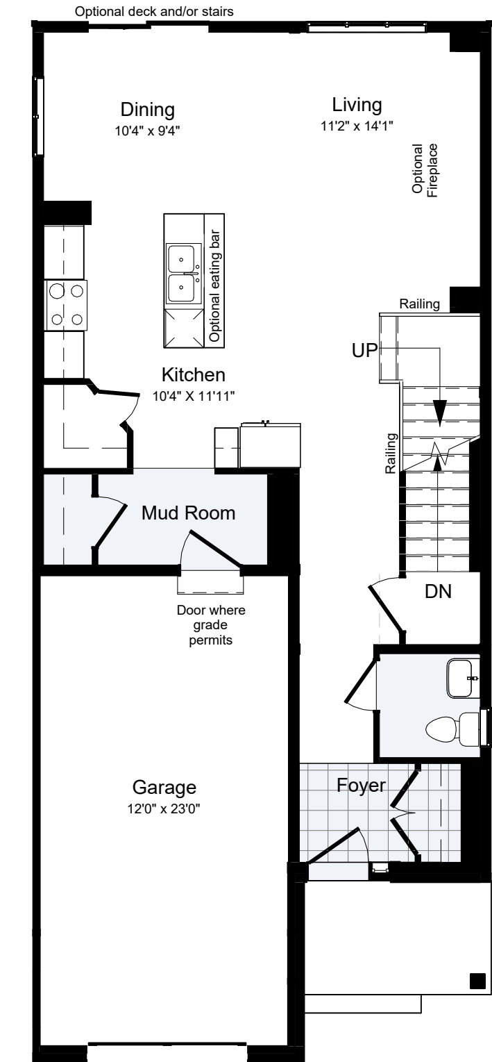
MAIN FLOOR
