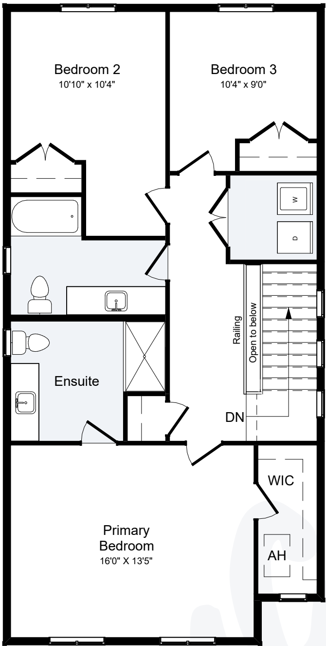
SECOND FLOOR
