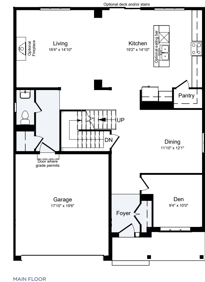
MAIN FLOOR
