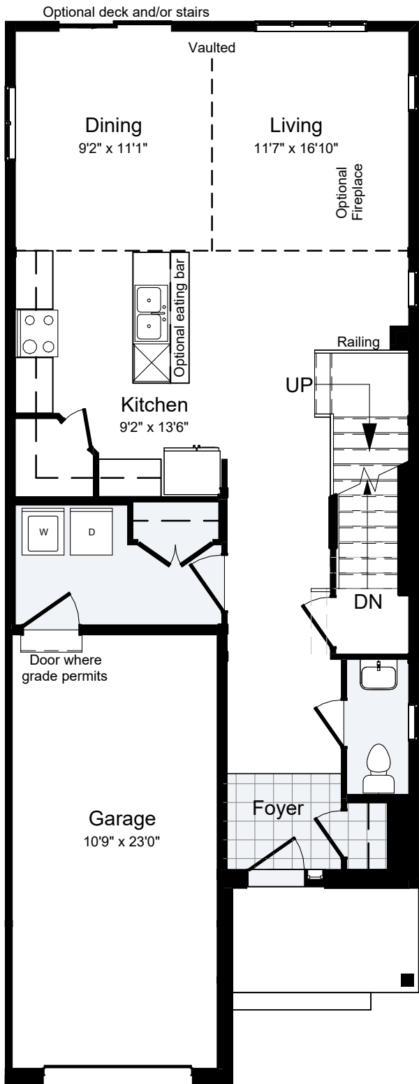
MAIN FLOOR
